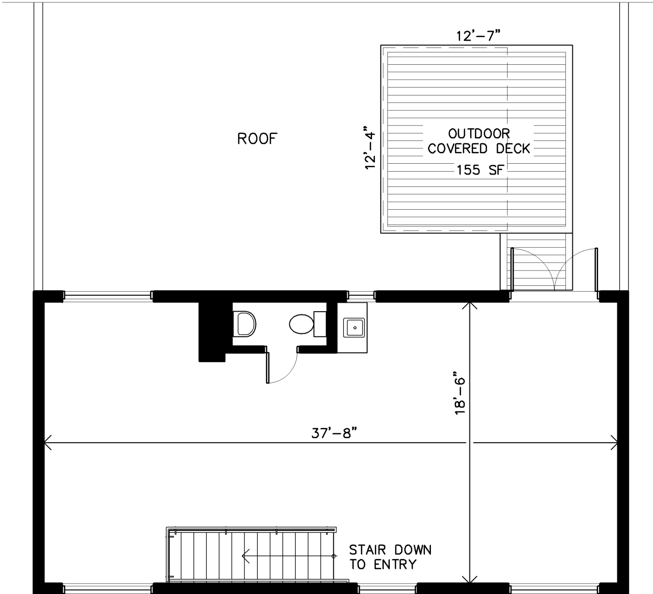
FLOOR 2 772.5 SF
