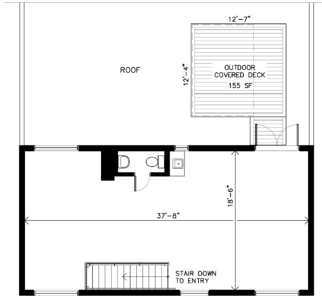
FLOOR 2 772.5 SF
